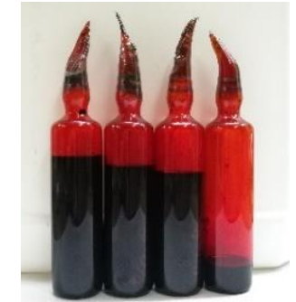
CrCl 2 O 2 (l)
