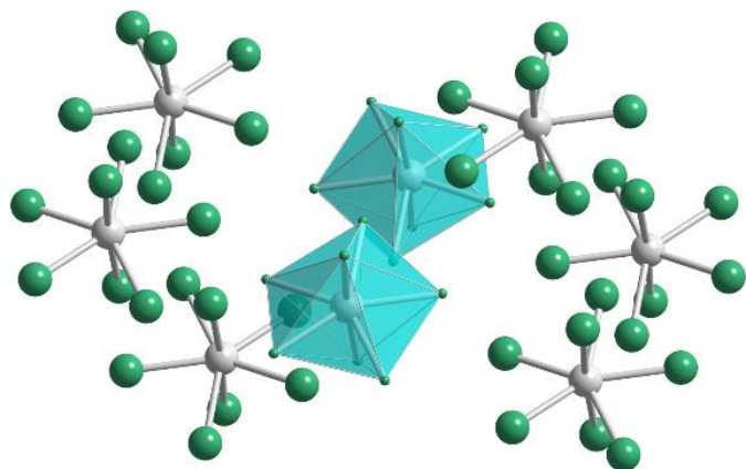
molekuly \text{ReF}_7
