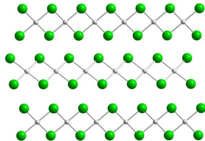
\alpha\text{-PdCl}_2
