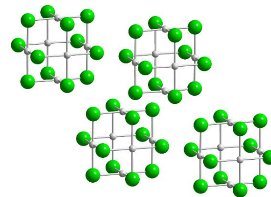
\beta\text{-PdCl}_2
