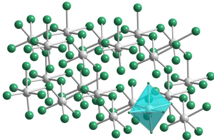
\text{PtF}_4
